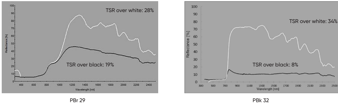
Figure 3: The role of surface color in TSR results Comparison of TSR values of PBr 29 and PBk 32 over white and black surfaces
