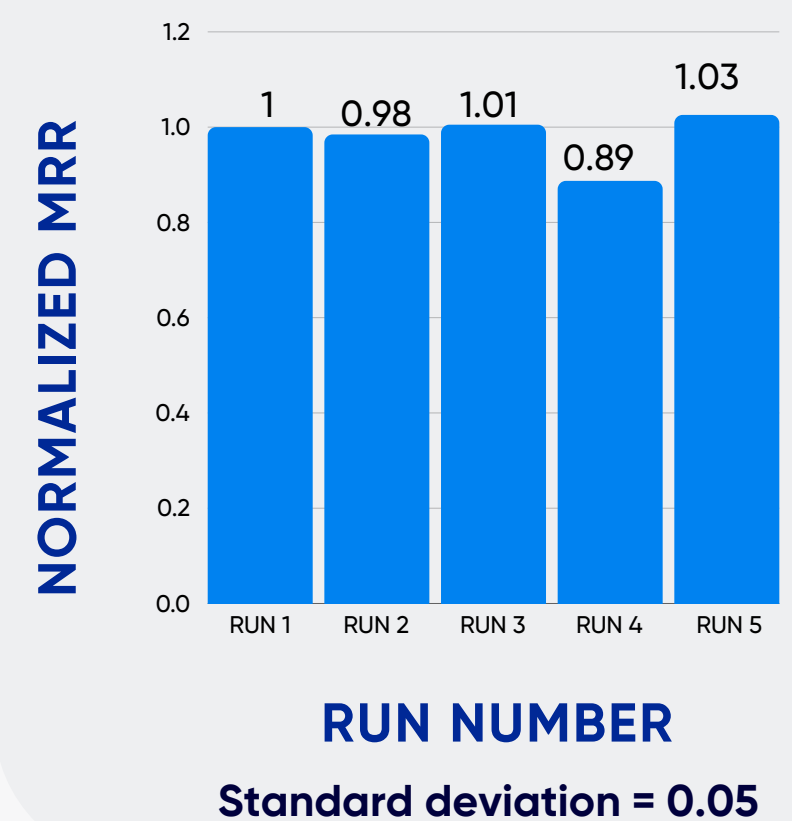
REPEATABILITY TEST
